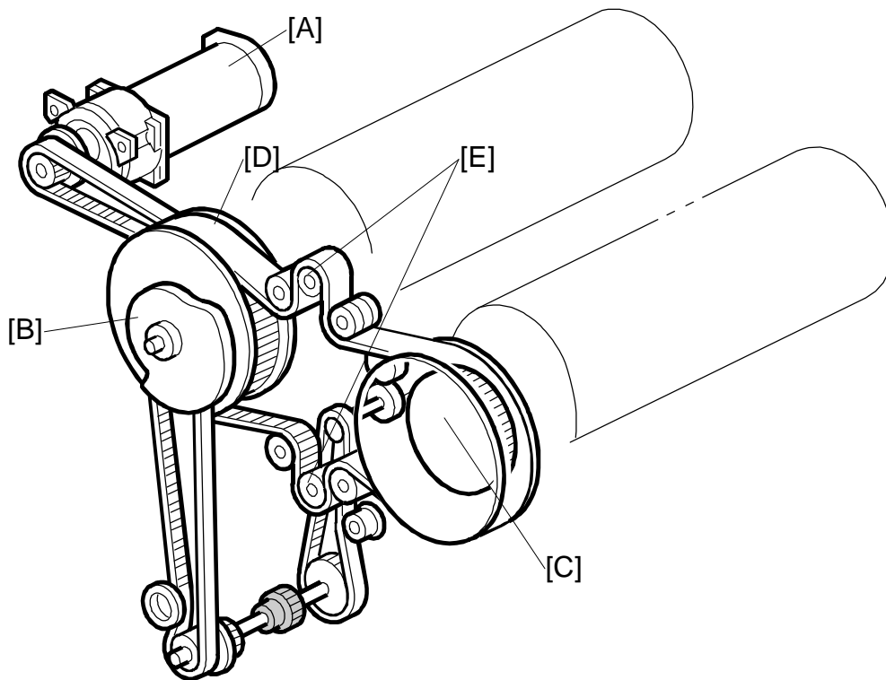
Rear view
